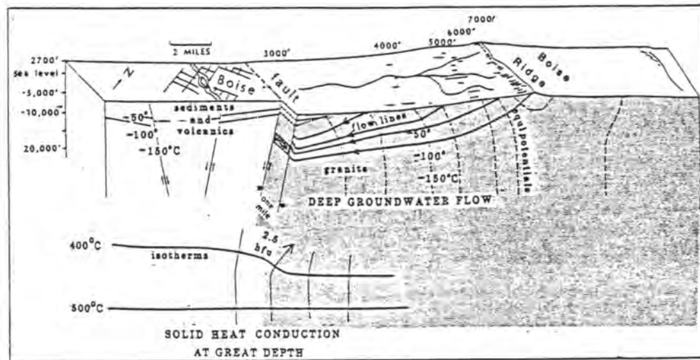
FIGURE 6. Conceptual model of the Boise geothermal system showing deep percolation of water in the granitic rocks driven by the regional topographic head of the mountains to the northeast. Solid conduction heat flow from great depth is refracted into the more conductive granite. Heat flow values are typically 2.5 HFU along the edge of the granitic highlands, and the gradient is typically 30^{\circ}\text{C}/\text{km} . Groundwater flow net is sketched using topography for equipotentials. Water must be driven to a depth of at least 2 km (7000 ft) in order to reach 75^{\circ}\text{C} . This constraint indicates a flow path of about 10 miles and a slope of 0.1 to 0.03. Radiocarbon ages of Boise geothermal waters range from 6000 to 12000 yrs (Mayo, 1983). Using a 7000 yr age and a flow path of 50,000 ft implies a flow rate of about 7 ft/yr, and a permeability of the granite 2 to 3 km deep of the order of 0.1 darcy. Discharge from a flow tube 2000 ft thick and one mile wide along the front would be about 1000 gal/min per linear mile along the front. Major objection to this kind of model is that it requires relatively high rock permeability of 0.1 darcy at a depth of 2 km. Permeabilities of crystalline rocks deeper than 1300 feet are more typically of the order of 0.001 darcy (Davis, 1981), but no data exists for the extensively fractured granitic rocks of the southern Idaho batholith along the margin of the Snake River Plain.
