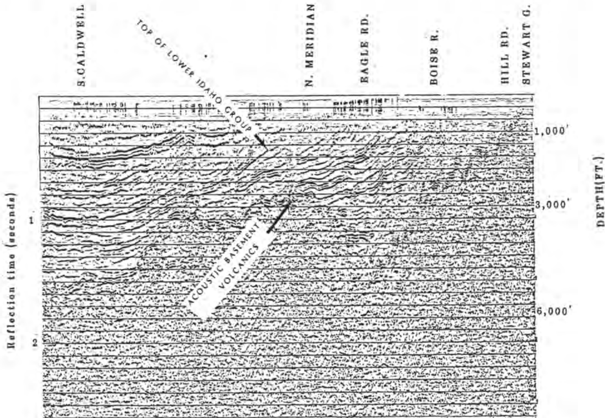
FIGURE 5. Seismic reflection section from the Boise foothills in Stewart Gulch to Caldwell, Idaho (35 miles). Location of section is shown on figure 1. Reflections above the acoustic basement are from sediments within the Idaho Group. Acoustic basement beneath the Meridian area is the top of a 7000-ft sequence of Miocene basalt described by Wood and Anderson (1981). Acoustic basement beneath Boise may be rhyolite or basalt. The section clearly shows the basin between Meridian and Boise filled by lower Idaho Group sediments. During the time of deposition of the upper Idaho Group the basin axis shifted southwest, and the upper Idaho Group fills a basin in the Caldwell area.
