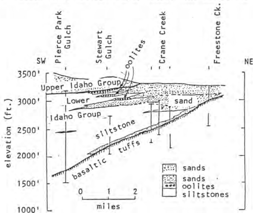
FIGURE 4. Stratigraphic section of the Idaho Group sediments in the Boise foothills compiled from water-well logs and geologic mapping. Vertical lines are locations of wells. Section illustrates the facies relationships of lake-margin sediments and the boundary between the upper and the lower Idaho Group.
