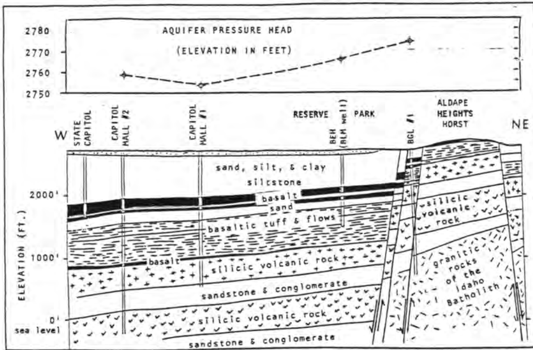
FIGURE 3. Geologic structure section across the main reservoir of the geothermal system constructed from well logs. Well locations are given in Table 1 and shown on fig. 2. Shown above the section is the piezometric level of water in the completed wells. Pressure is shown as elevation of the column of hot water in the well and prior to significant production. Section is true scale--no vertical exaggeration.
